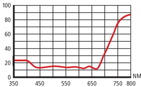
Resin Glas GND Kurve
