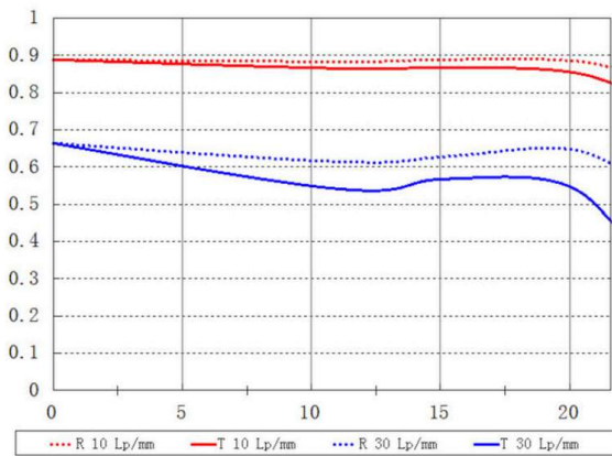
MTF-Kurven
