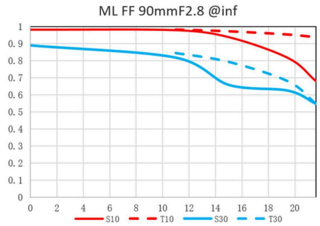
MTF-Kurve
