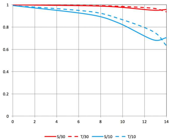
MTF-Kurven
