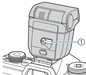
① ON/OFF-Schalter
